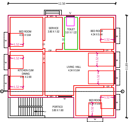
PRO. GROUND FLOOR PLAN.
