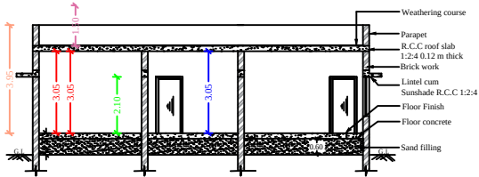
SECTION "N-R"
