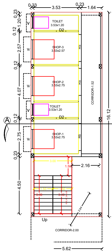
D FLOOR PLAN
