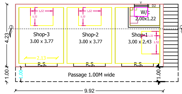
PRO.GROUND FLOOR PLAN
