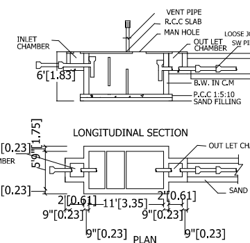
SEPTIC TANK
