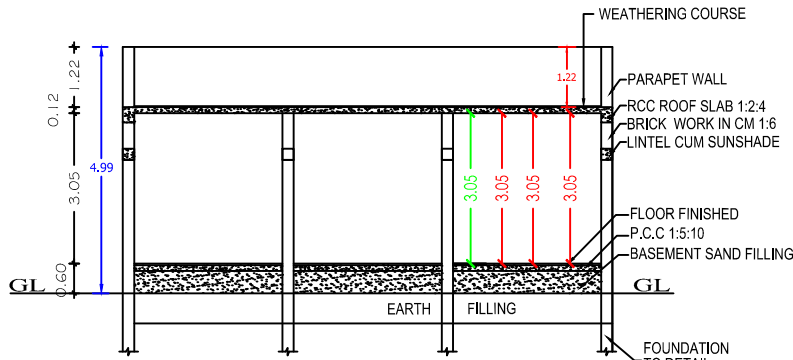
SECTION ON "J-J"
