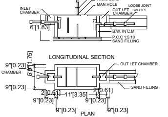
RAIN WATER HARVESTING SYSTEM RWV_CAPACITY_L=1000LTRS
