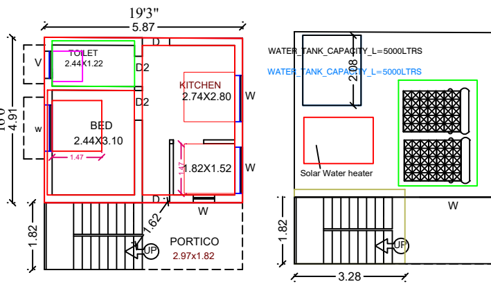
GROUND FLOOR PLAN TERRACE FLOOR PLAN
