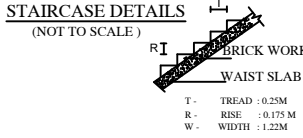
STAIRCASE DETAILS (NOT TO SCALE)
