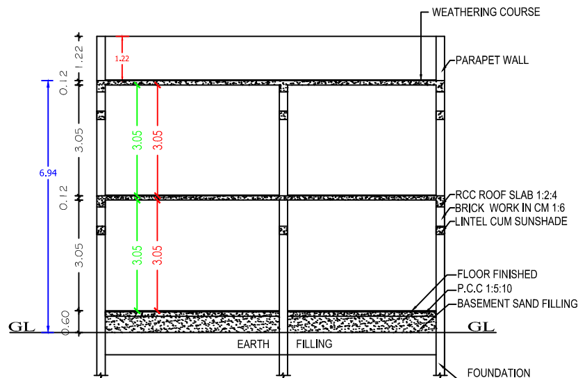
SECTION ON "J-J"
