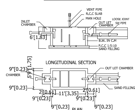
SEPTIC TANK
