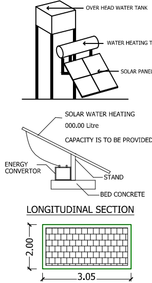
SOLAR SYSTEM
