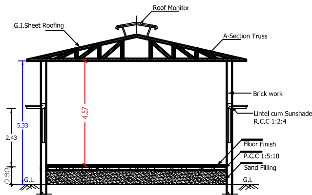
SECTION ON "J-J"
