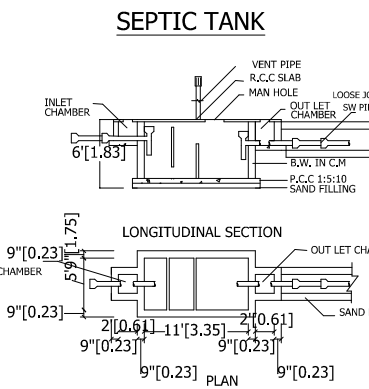
SEPTIC TANK
