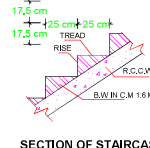
SECTION OF STAIRCASE
