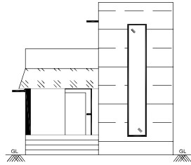
FRONT ELEVATION
