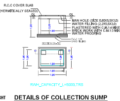
DETAILS OF COLLECTION SUMP FOR RAIN PLAN
