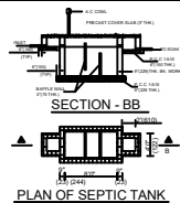
PLAN OF SEPTIC TANK
