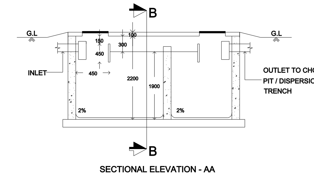
SECTIONAL ELEVATION - AA
