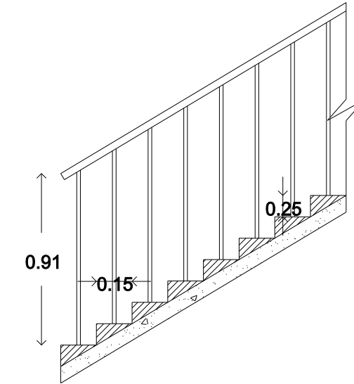
STAIRCASE DETAILS
