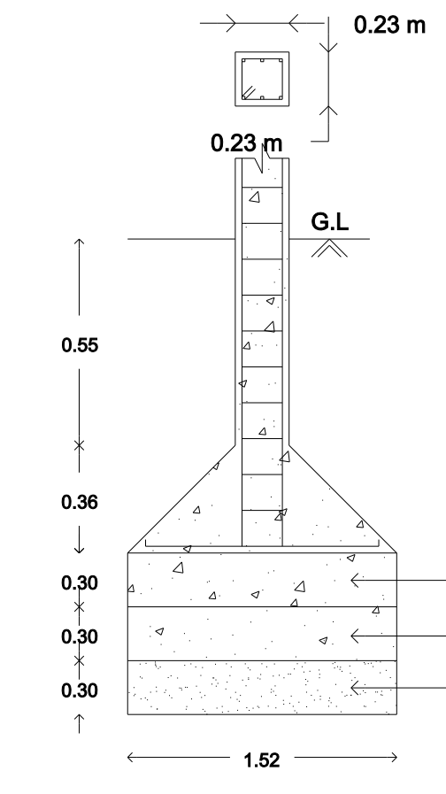
FOUNDATION DETAILS
