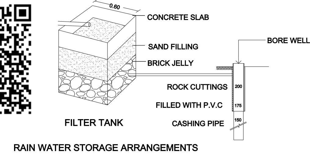
RAIN WATER STORAGE ARRANGEMENTS
