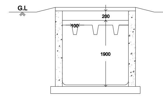
SECTIONAL ELEVATION - BB
