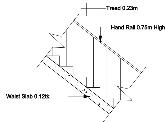
STAIR DETAILS SCALE : 1:50
