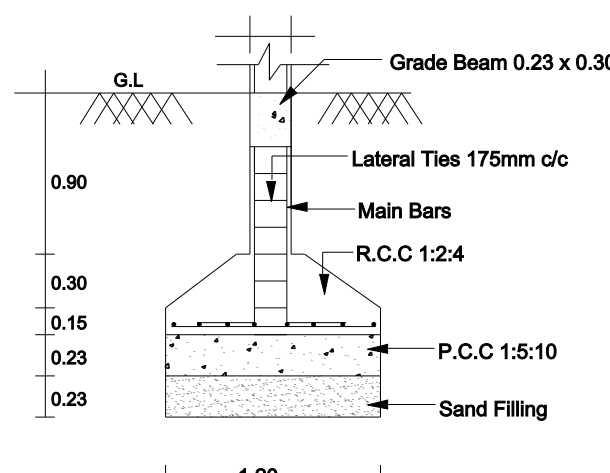
FOOTING DETAILS SCALE : NOT TO SCALE
