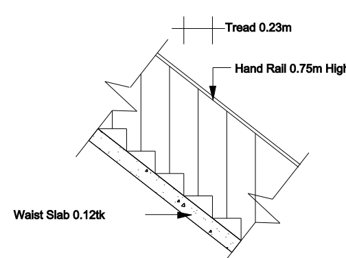
STAIR DETAILS SCALE : 1:50
