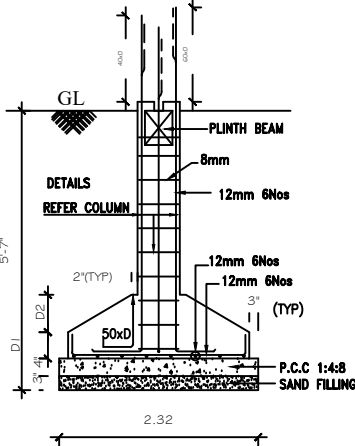
FOUNDATION DETAILS
