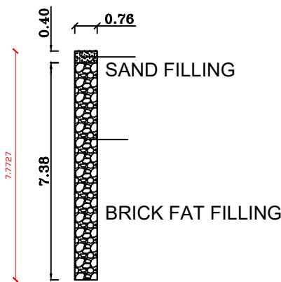
DETAILS OF PERCOLATION PIT
