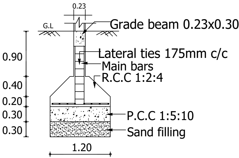
FOOTING DETAILS SCALE 1:50
