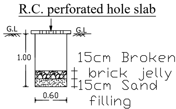
RAIN WATER HARVEST PIT SCALE 1:50
