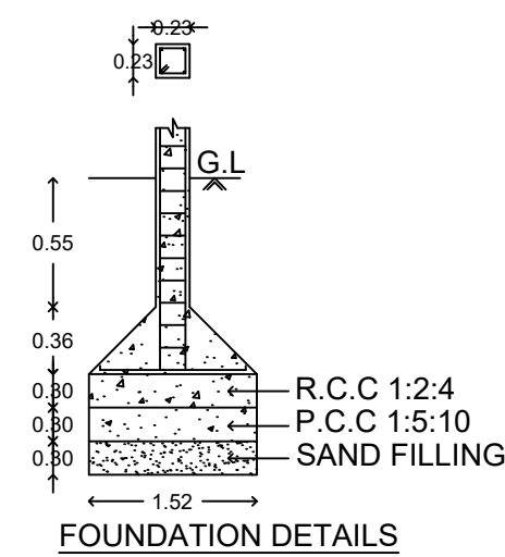
FOUNDATION DETAILS
