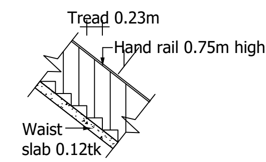
STAIR DETAILS
