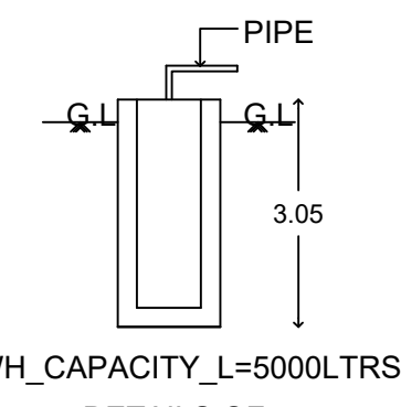
DETAILS OF RAINWATER COLLECTION TANK
