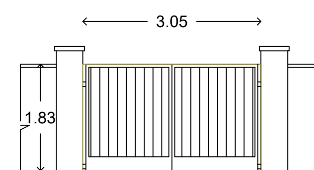
MAIN GATE
