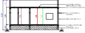
SECTION - "AB"
