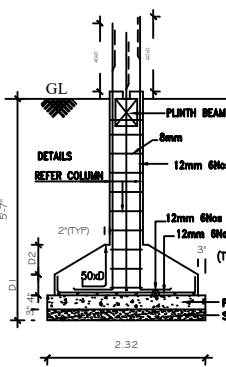
FOUNDATION DETAILS SCALE : 1:50.
