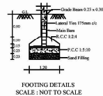
FOOTING DETAILS SCALE: NOT TO SCALE
