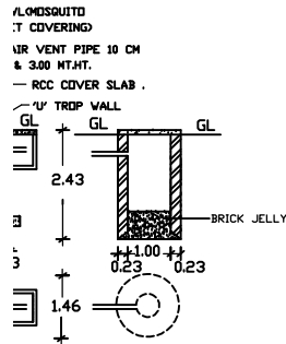
PLAN AND CROSS SECTION OF ST&SP
