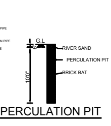
PERCOLATION PIT
