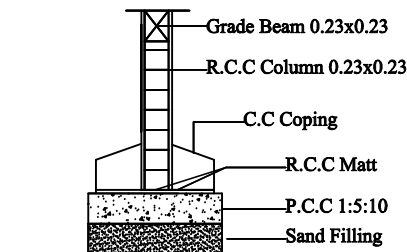
Foundation Details
