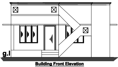
Building Front Elevation
