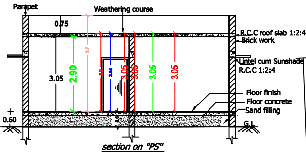
section on "PS"
