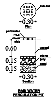
RAIN WATER PERCUSSION PIT
