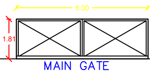
MAIN GATE
