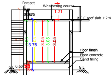
SECTION ON KR
