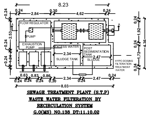
SEWAGE TREATMENT PLANT (S.T.P)
