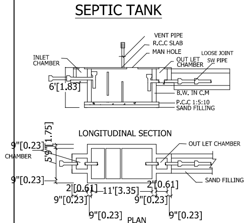
SEPTIC TANK
