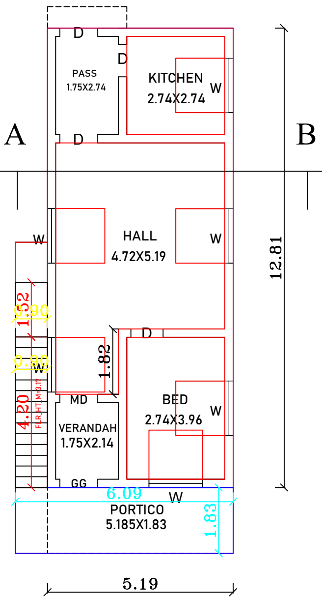
PRO G FLOOR PLAN
