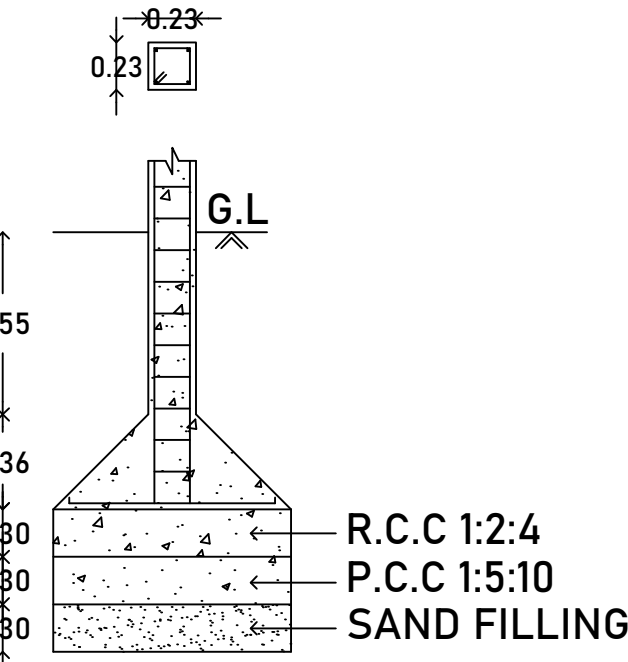
FOUNDATION DETAILS
