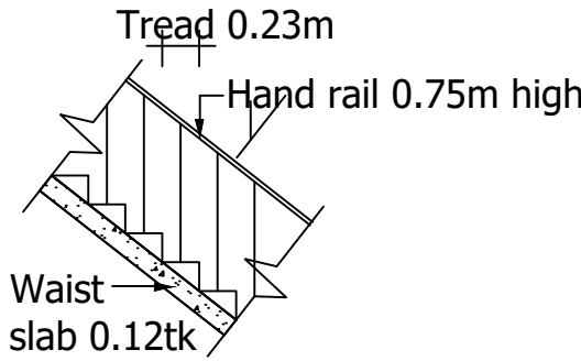
STAIR DETAILS
