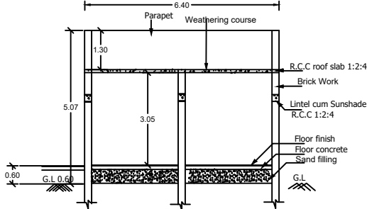
SECTION ON "A S"
