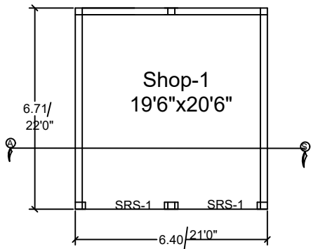
PROPOSED G.F. PLAN.
