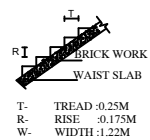
STAIRCASE DETAILS (NOT TO SCALE)
