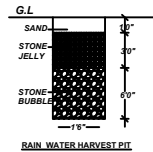
RAIN WATER HARVEST PIT
