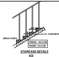
STAIRCASE DETAILS N/S
