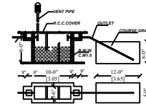
SEPTIC TANK & D-TRENCH DETAILS (NOT TO SCALE)
