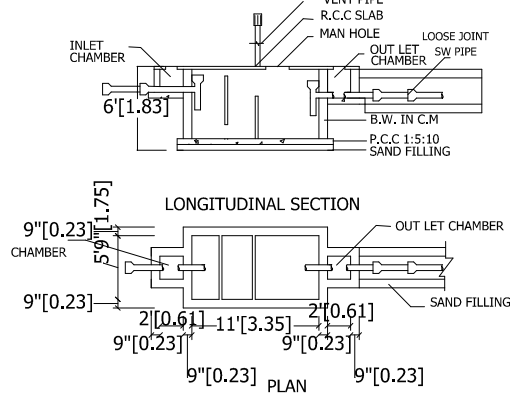
SEPTIC TANK
