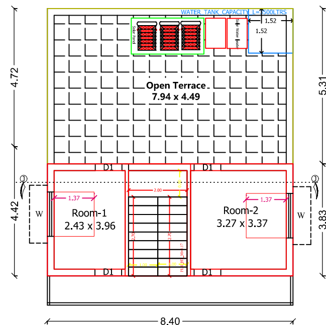
PRO.FIRST FLOOR PLAN
