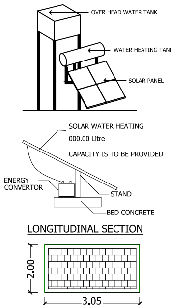
SOLAR SYSTEM
