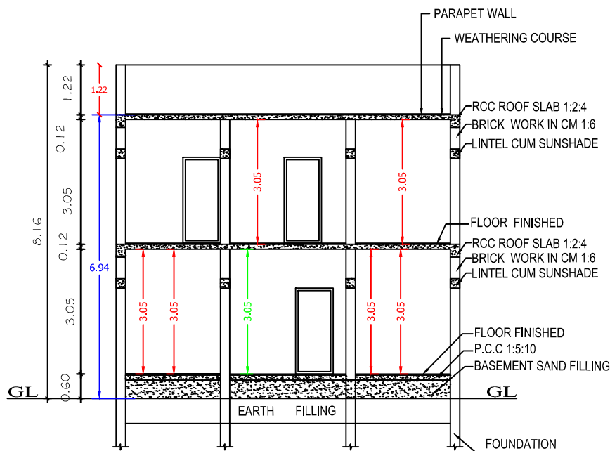
SECTION ON "J-J"
