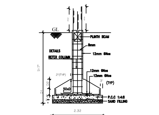
FOUNDATION DETAILS
