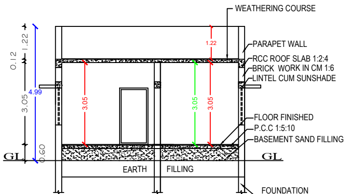
SECTION ON "J-J"
