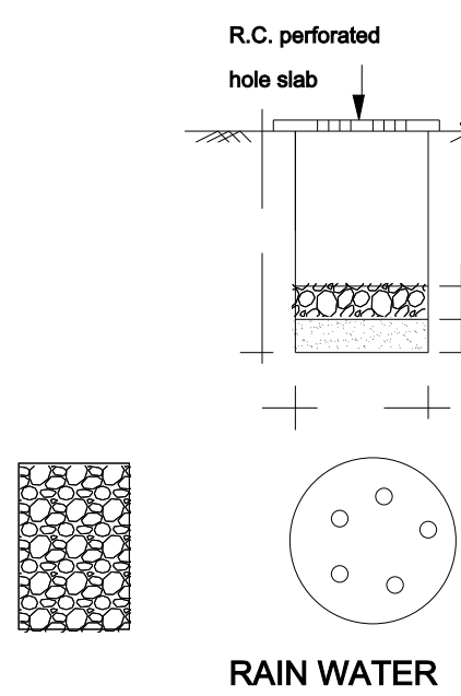
RAIN WATER
