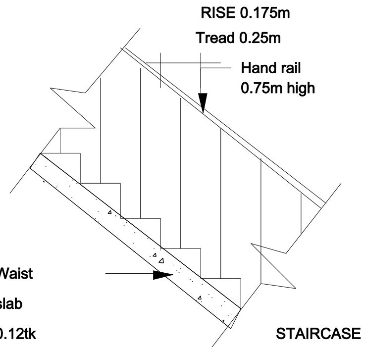
STAIRCASE
