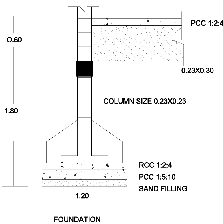
FOUNDATION
