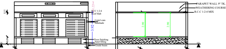
FRONT ELEVATION
