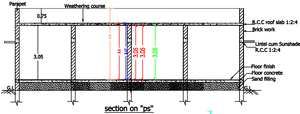
section on "ps"
