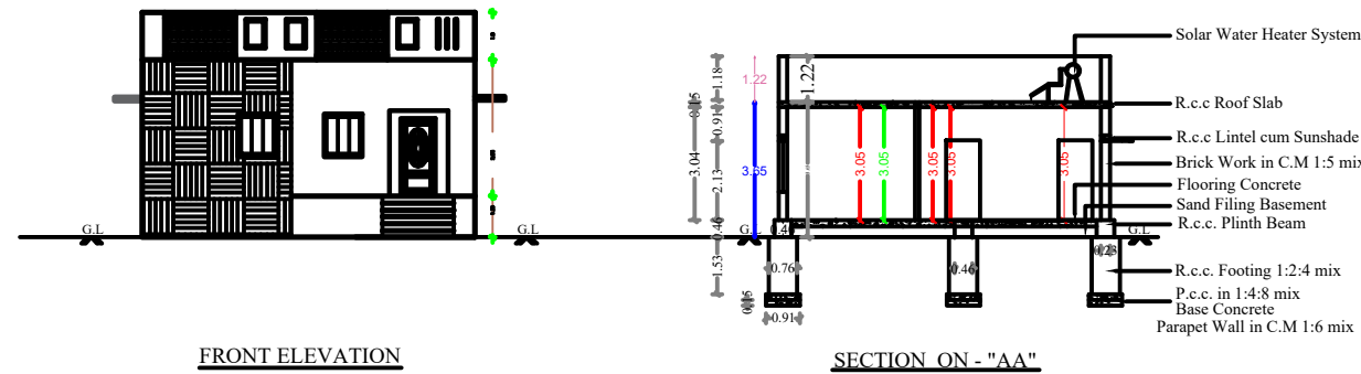
FRONT ELEVATION
