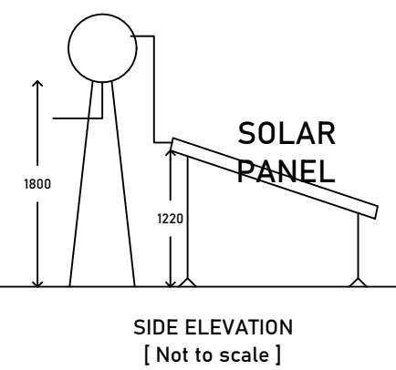
SOLAR WATER HEATER [ NOT TO SCALE ]
