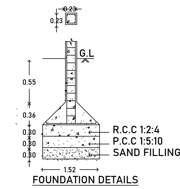
FOUNDATION DETAILS
