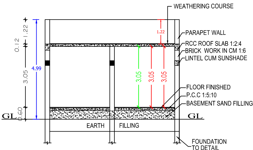
SECTION ON "J-J"
