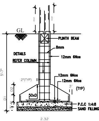
FOUNDATION DETAILS
