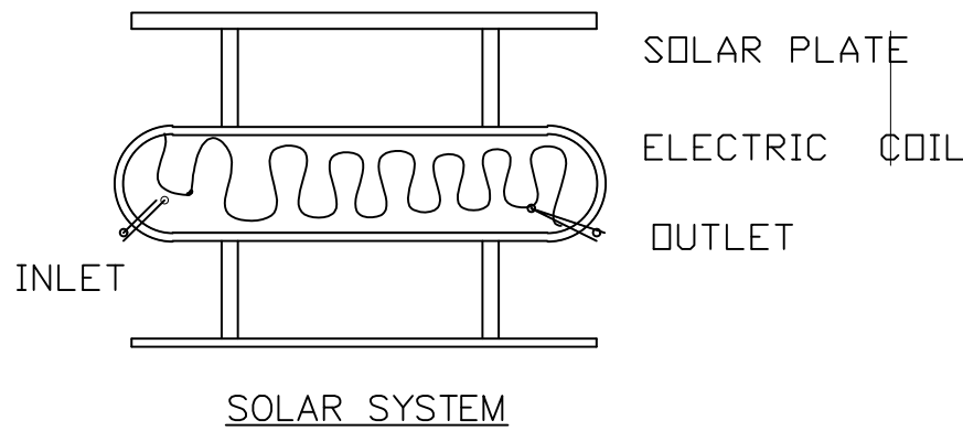
SOLAR SYSTEM
