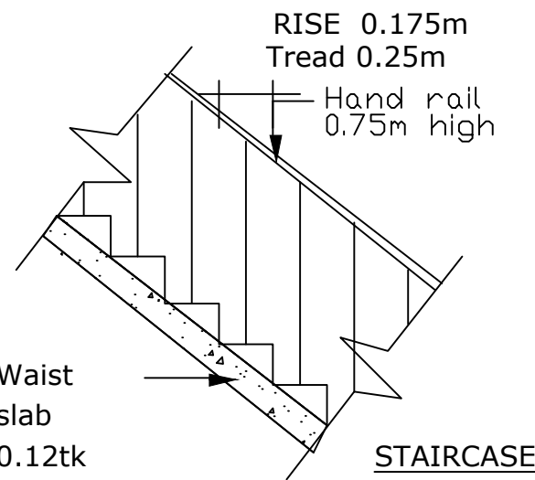
STAIRCASE
