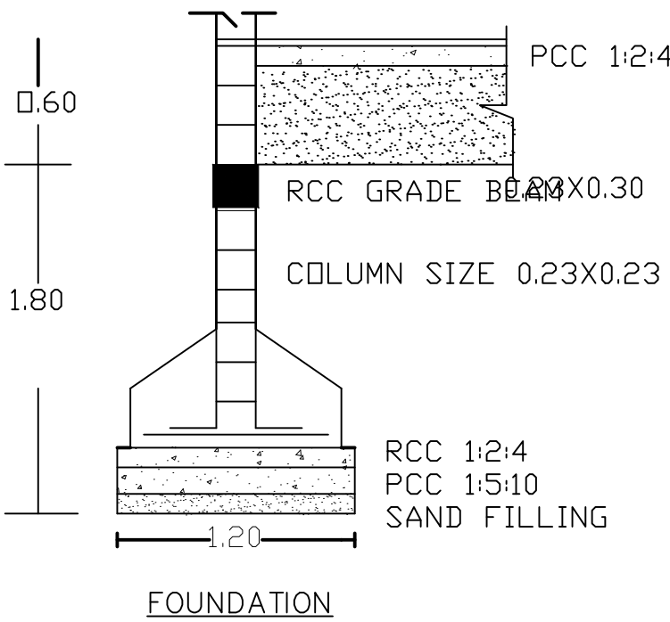
FOUNDATION
