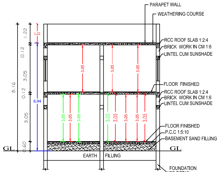
SECTION ON "J-J"
