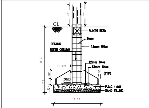
FOUNDATION DETAIL
