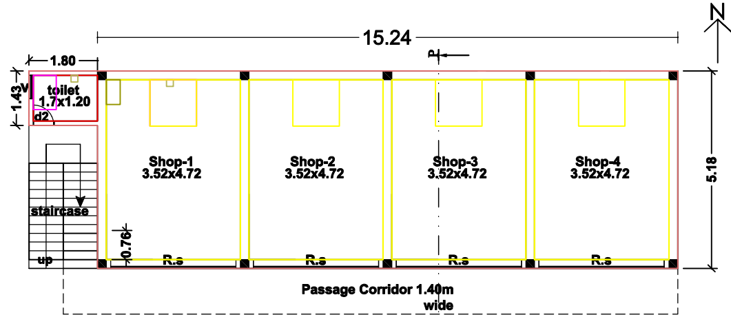
Proposed g.f Building plan
