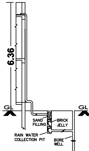
RAIN WATER HARVESTING SYSTEM RWH_CAPACITY_L=1000LTRS
