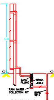
RAIN WATER HARVESTING SYSTEM RWHL_CAPACITY_L=1000LTRS
