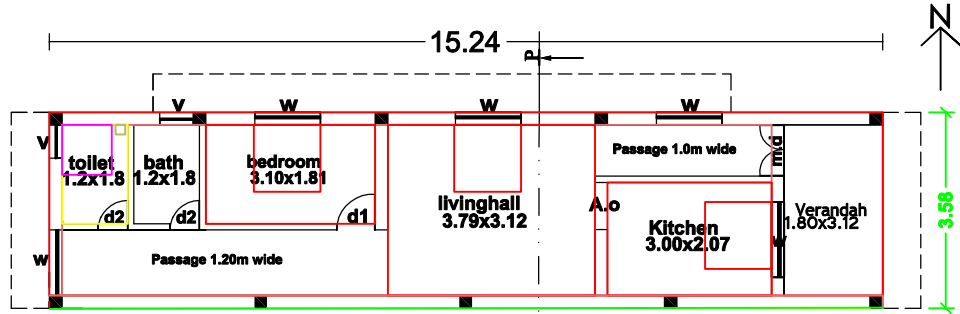
Proposed g.f Building plan
