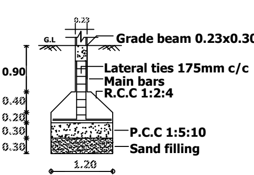
FOOTING DETAILS SCALE 1:50
