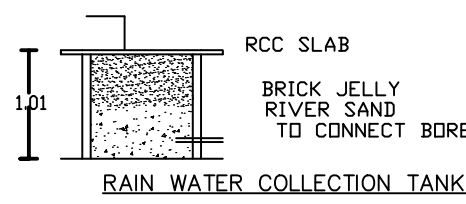
RAIN WATER COLLECTION TANK
