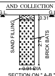
SECTION ON "A-B"
