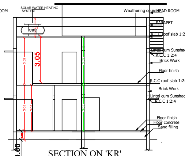
SECTION ON 'KR'
