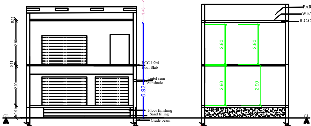
ELEVATION SECTION A-A
