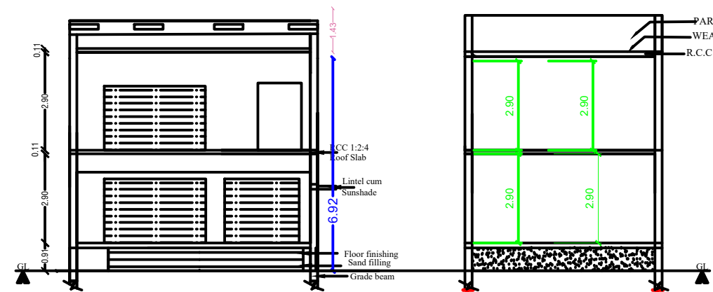
ELEVATION SECTION A-A
