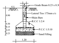
FOOTING DETAILS SCALE : NOT TO SCALE
