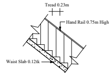
STAIR DETAILS SCALE : NOT TO SCALE
