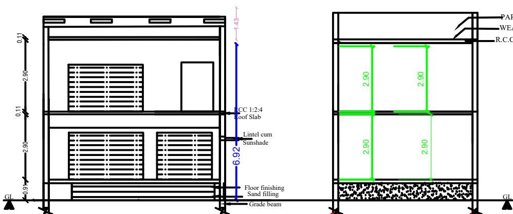
ELEVATION SECTION A-A
