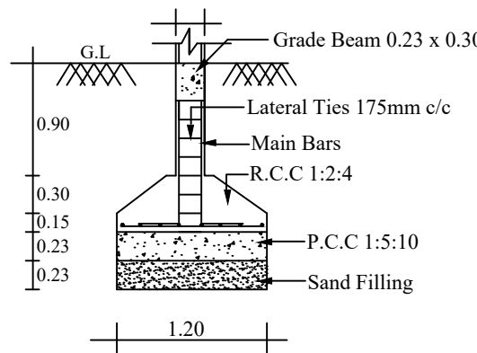
FOOTING DETAILS SCALE : NOT TO SCALE
