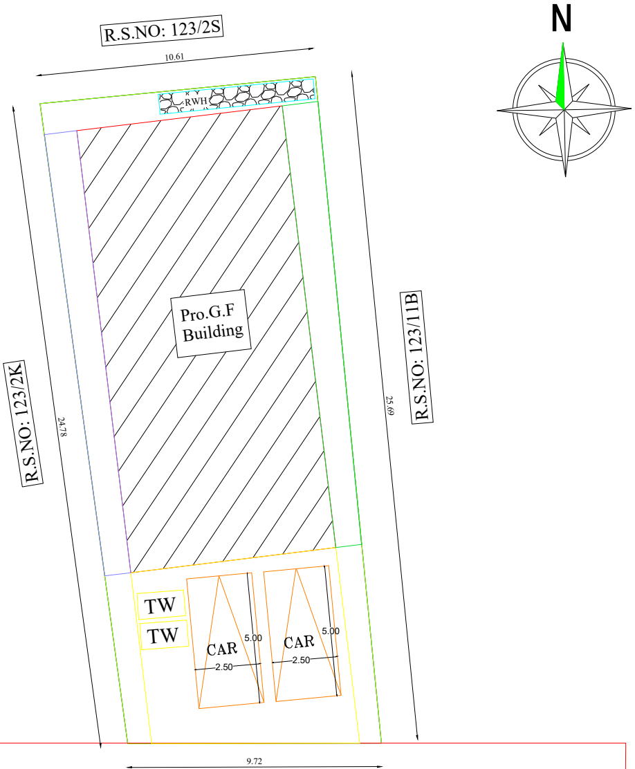
Ex. Road SITE PLAN SCALE 1:100
