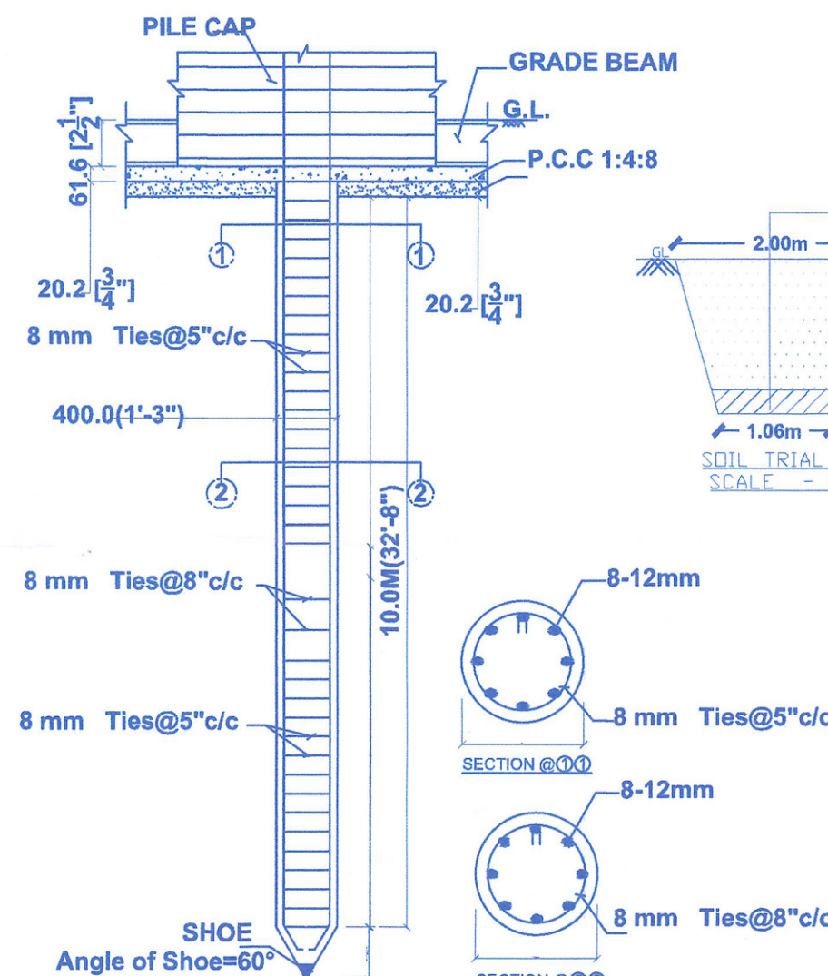
LONGITUDINAL SECTION OF PILE
