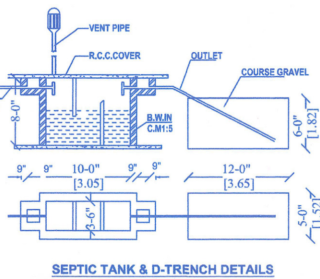
SEPTIC TANK & D-TRENCH DETAILS (NOT TO SCALE)
