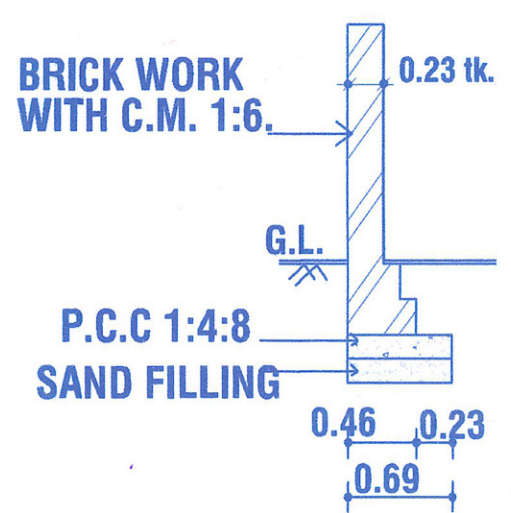
BRICK WORK WITH C.M. 1:6 P.C.C 1:4:8 SAND FILLING
