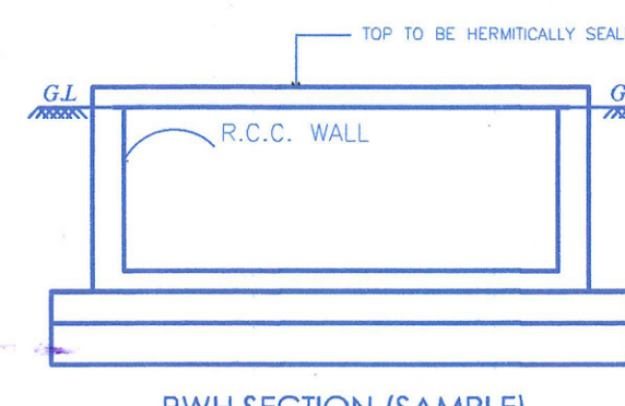
RWH SECTION (SAMPLE)
