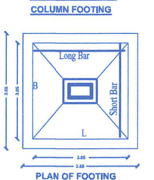
PLAN OF FOOTING
