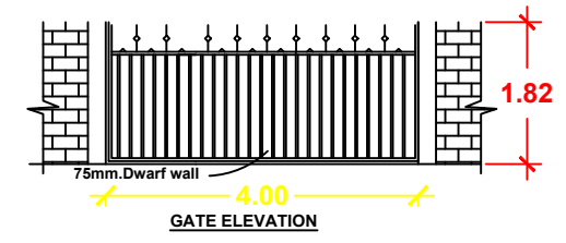
GATE ELEVATION
