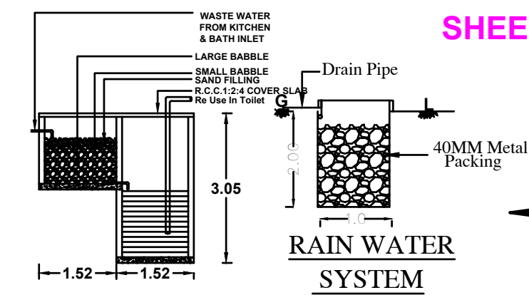
RECYCLING OF WASTE WATER FROM KITCHEN & BATHROOM
