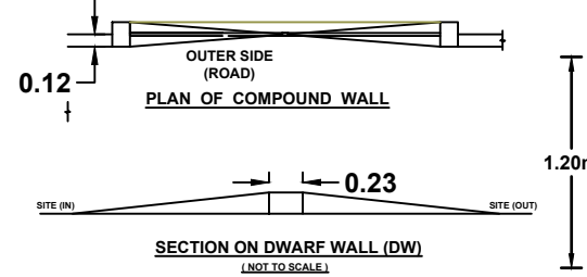
SECTION ON DWARF WALL (DW) ( NOT TO SCALE )
